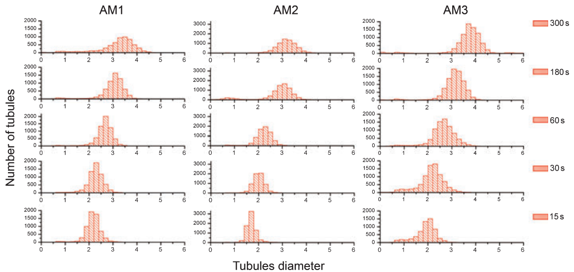
Figure 10 Minimum tubule diameter histograms of 16 fields for each sample against time.
