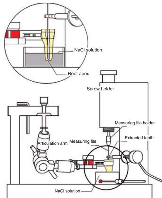
Figure 1 Measuring unit.
