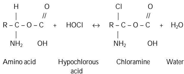
Scheme 3. Chloramination reaction.
