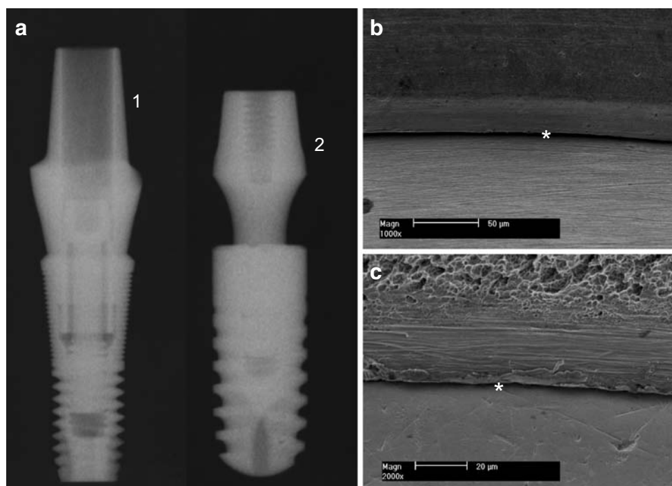
Fig. 1 a X-ray pictures of MicroThread-OsseoSpeed implant bolted with TiDesign Abutment (AstraTech) (1) and Ankylos Plus implant bolted with straight standard abutment (2). b Scanning electron microscope picture of the implant-abutment connection (AstraTech). c Scanning electron microscopy photo of the implant-abutment connection (Ankylos). The marginal gap between implant and abutment is marked with a star
